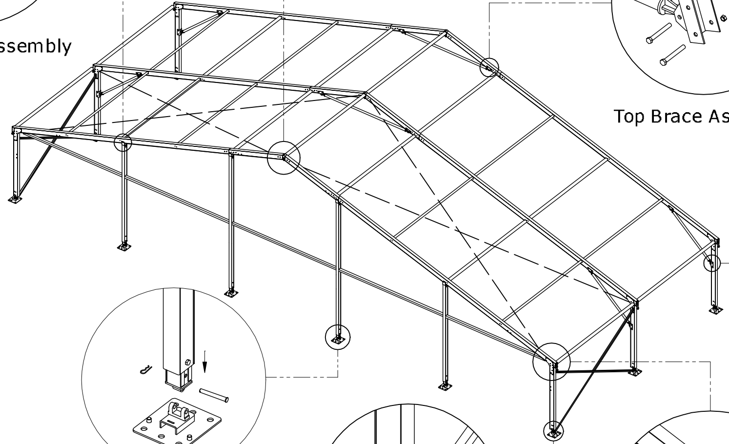
Gable Pole/ Baseplate Assembly
