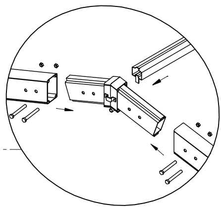
Ridge Assembly
