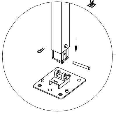
Gable Pole/ Baseplate Assembly
