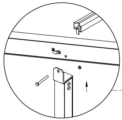
Gable Pole Assembly
