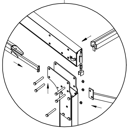
Corner Assembly
