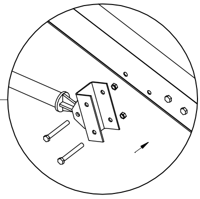
Top Brace Assembly
