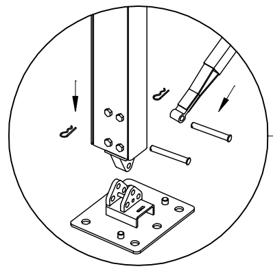
Upright Support/ Baseplate/Cross Bar Assembly
