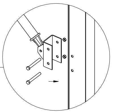
Upright Support/ Corner Brace Assembly
